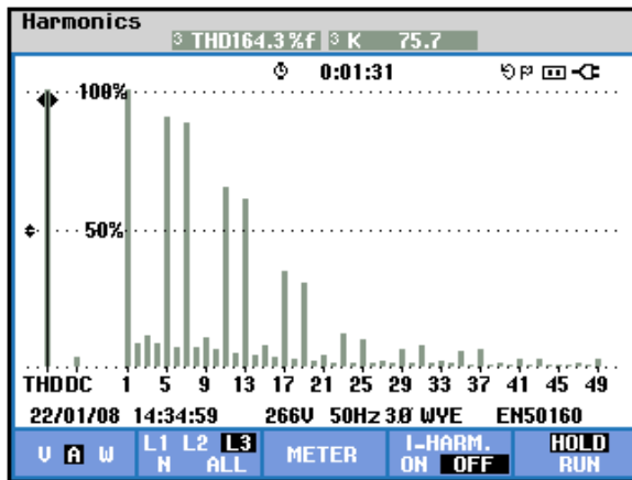
Current harmonics THD = 164.3% (scale 0-100%)
