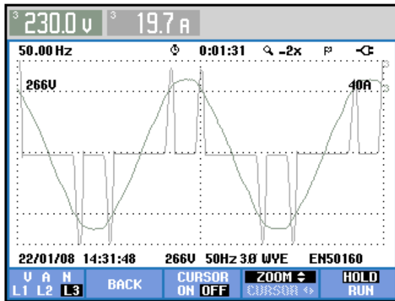
Voltage and current waveforms
