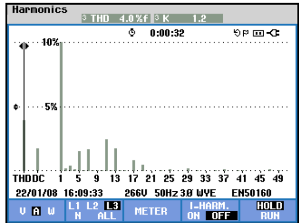
Current Harmonics THD = 4.0% (scale 0-10%)
